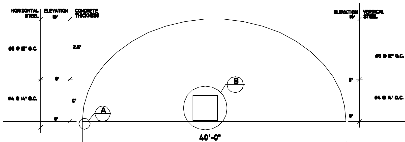
STEEL SCHEDULE - 40'x16' DOME
