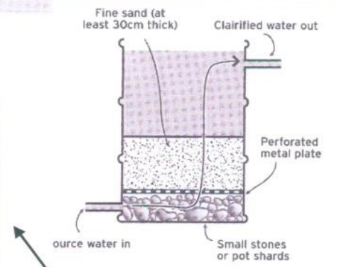
FIGURE 12c: GRAVITY-FED WATER FILTERING SYSTEM
