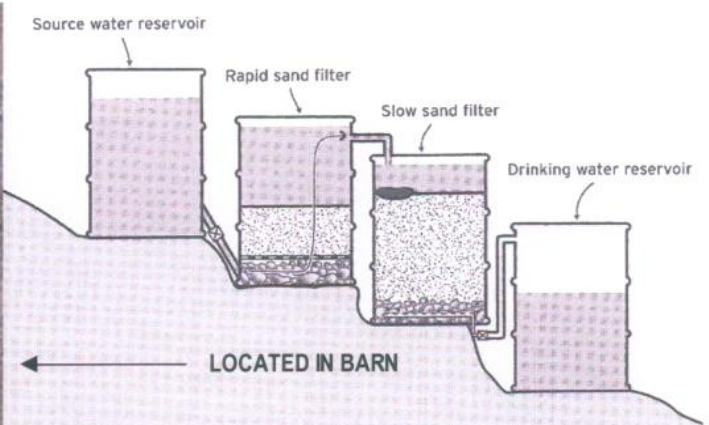
FIGURE 12c: GRAVITY-FED WATER FILTERING SYSTEM
