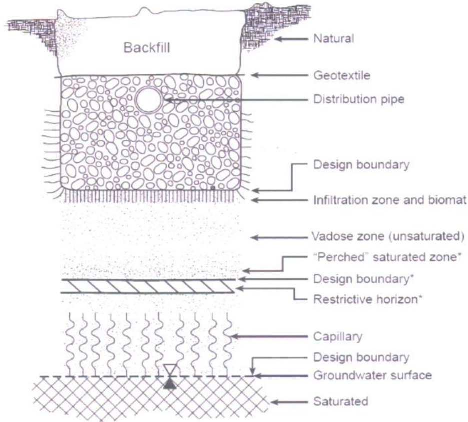
Figure 5-3. Subsurface wastewater infiltration system design/performance boundaries.
