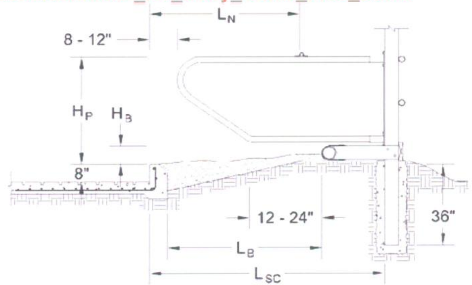
Closed Front Freestall with Generous Bedding
